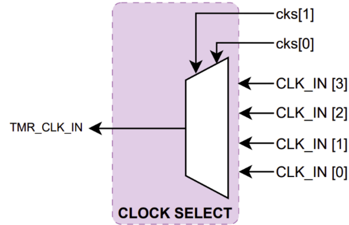
Figure CLOCK SELECT Block diagram
